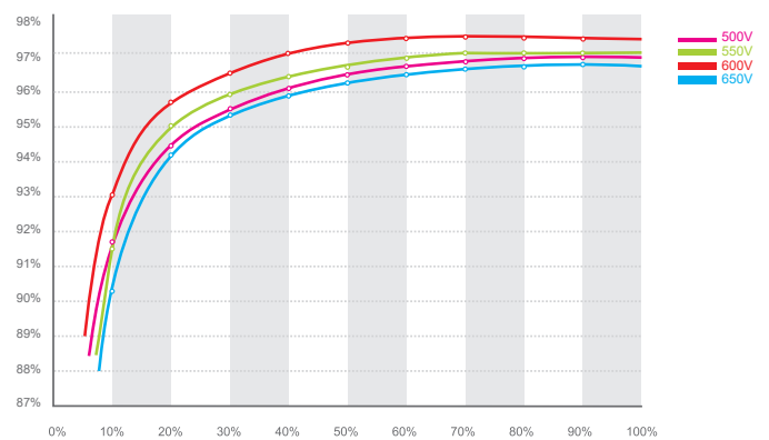
Growatt 6000UE efficiency
